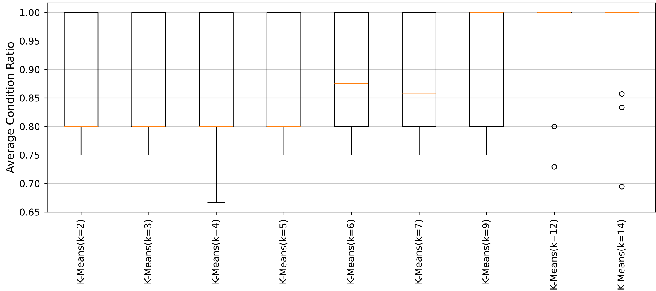
YARA Rules Average Condition Ratio Distribution (Cluster7_Size14 dataset)
